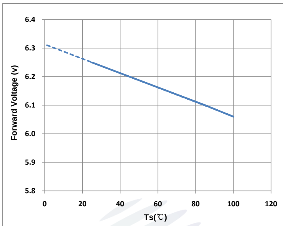
Fig 1-11 Forward Voltage Vs Solder Temperature 电压与管脚温度特性曲线
