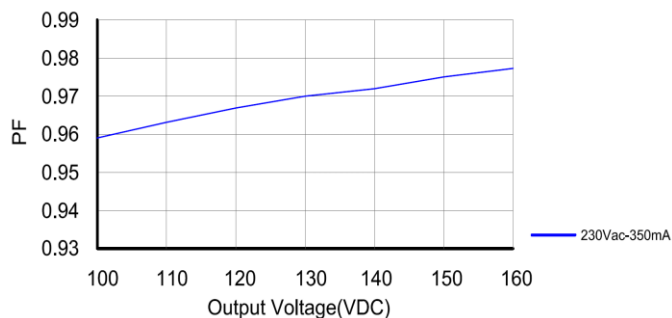
Power Factor Characteristics
