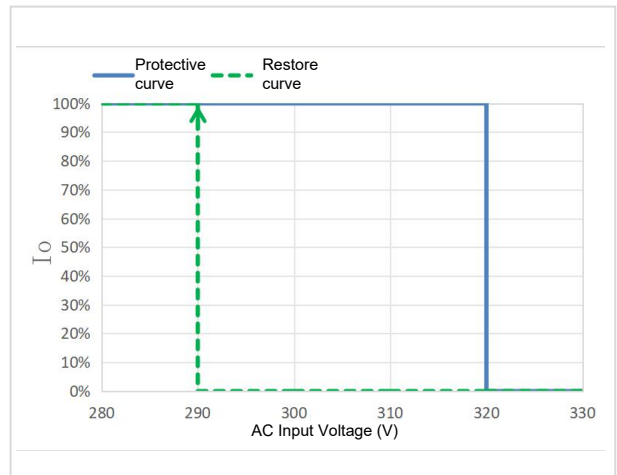
Schematic Diagram of Input Overvoltage Protection
