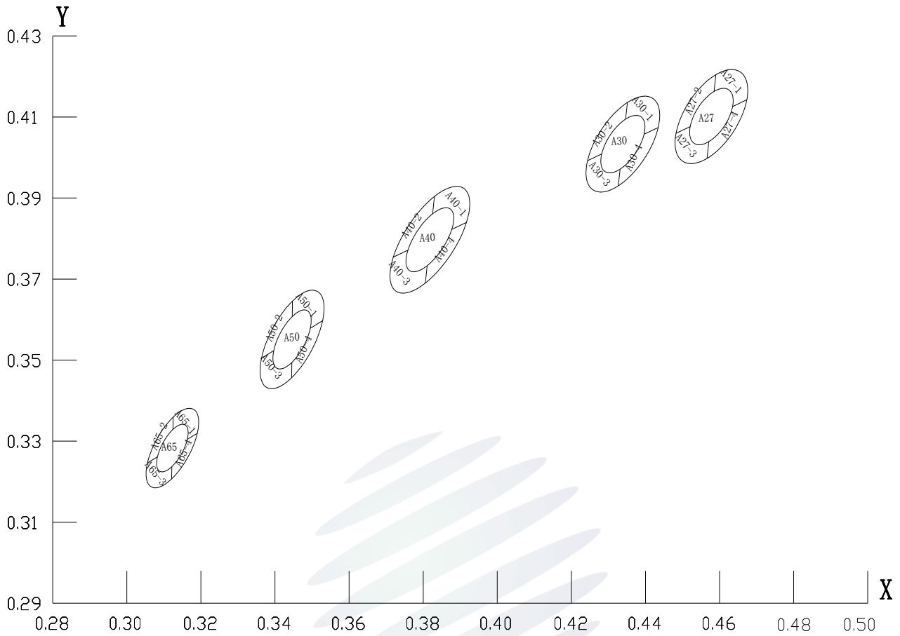
Fig 1-6 The C.I.E Chromaticity Diagram CIE色度
