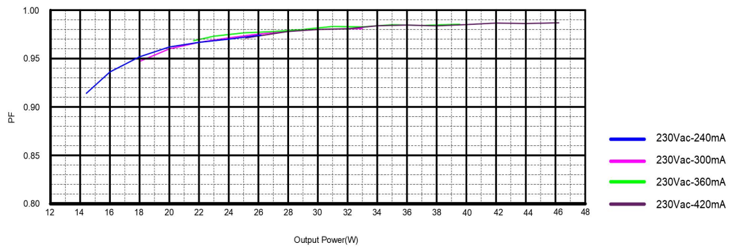
Power Factor Characteristics
