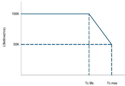
Lifetime vs. Temperature Curve
