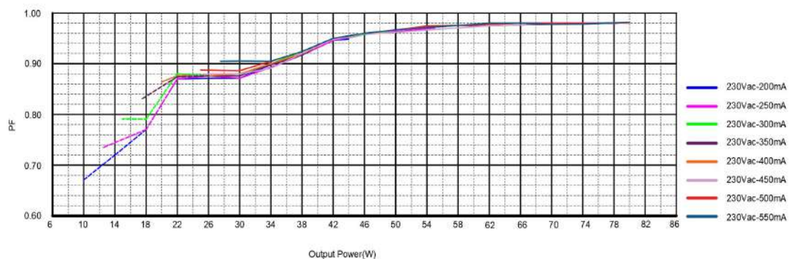
Power Factor Characteristics
