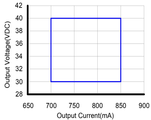
Operating window
