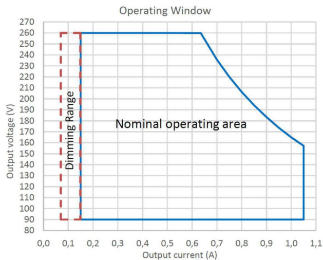
OT 165 1A0 NFC G3 Operating Window
